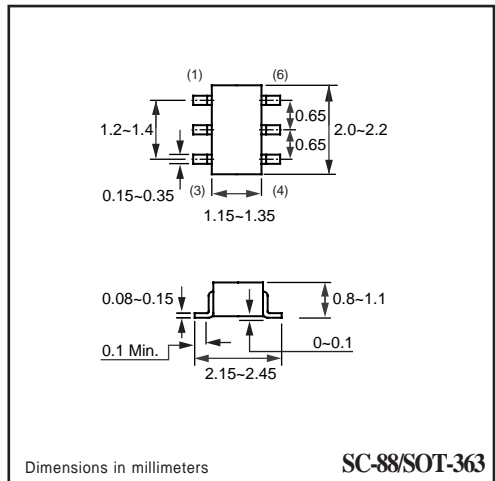
SC-88/SOT-363
